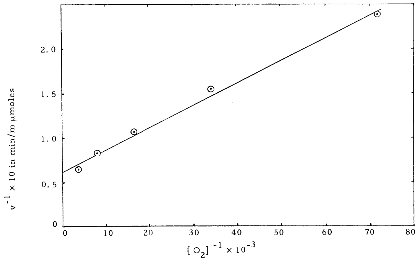
Figure 4. Lineweaver-Burk plot of the influence of oxygen tension on the rate of tryptamine oxidation by diamine oxidase (DAO) at pH 8. Tryptamine, 205 m \mu moles, and 0.05 mg of DAO were incubated in a total volume of 1.1 ml. (For a discussion of Lineweaver-Burk plots, see Mähler and Cordes, 1966, p. 228).
