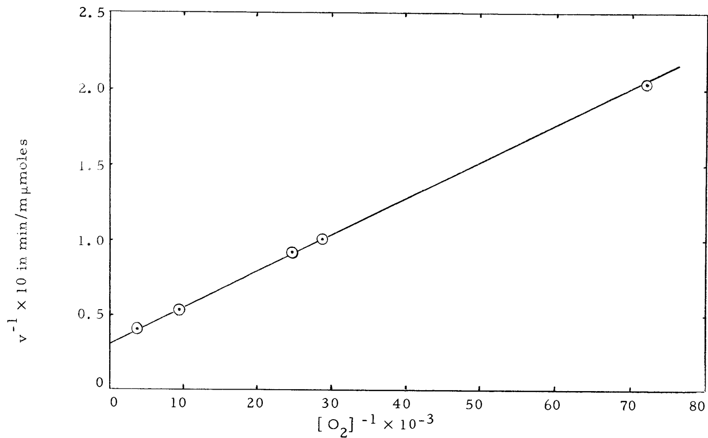
Figure 5. Lineweaver-Burk plot of the influence of oxygen tension on the rate of tryptamine oxidation by diamine oxidase (DAO) at pH 8. Tryptamine, 1000 m \mu moles, and 0.05 mg of DAO were incubated in a total volume of 1.1 ml.
