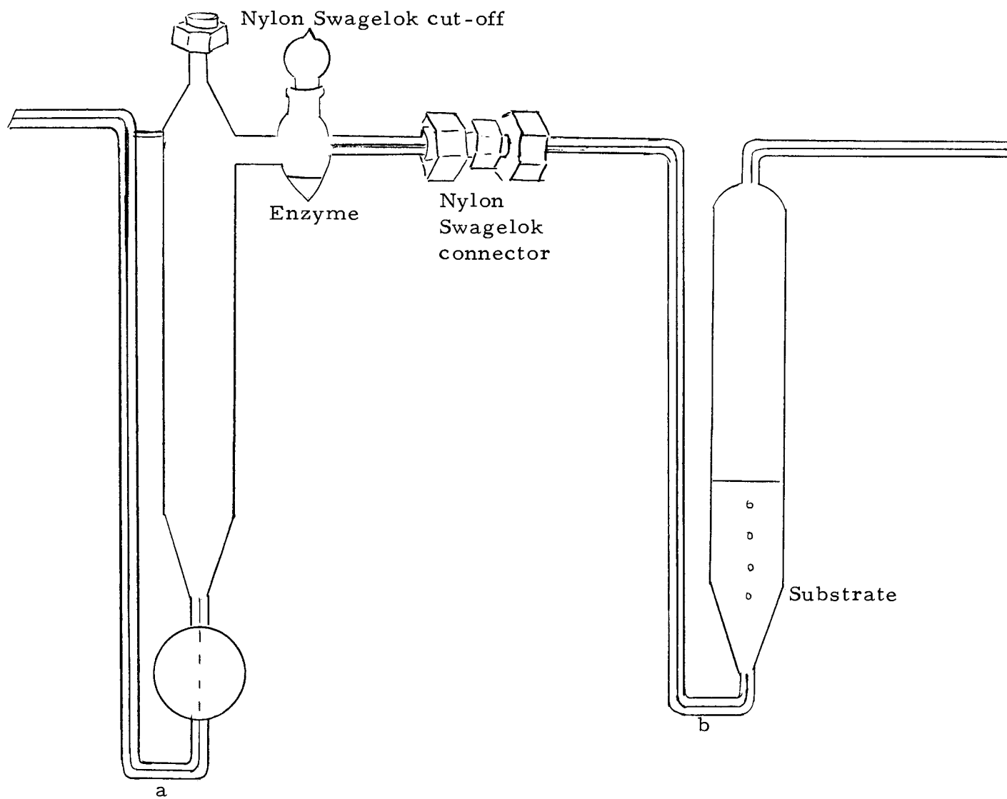
Figure 3. Diagrams of a-enzyme-reaction vessel and b-substrate vessel.
