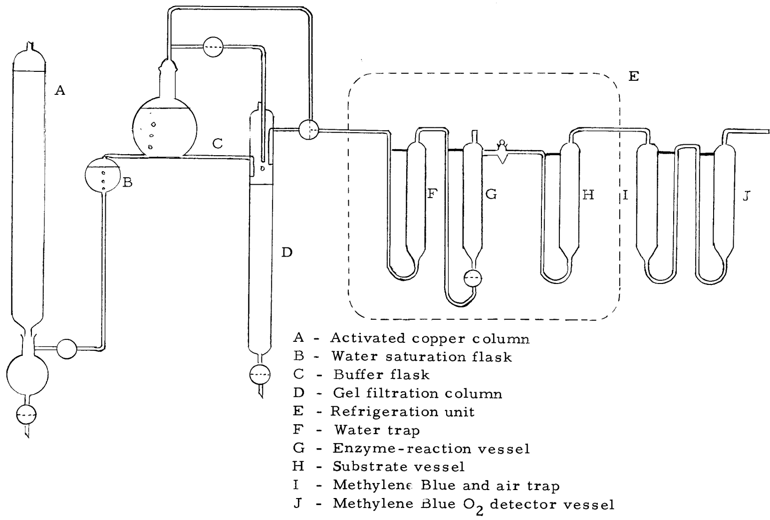
Figure 2. Diagram of system for running enzyme reactions in an O 2 -free N 2 atmosphere.
