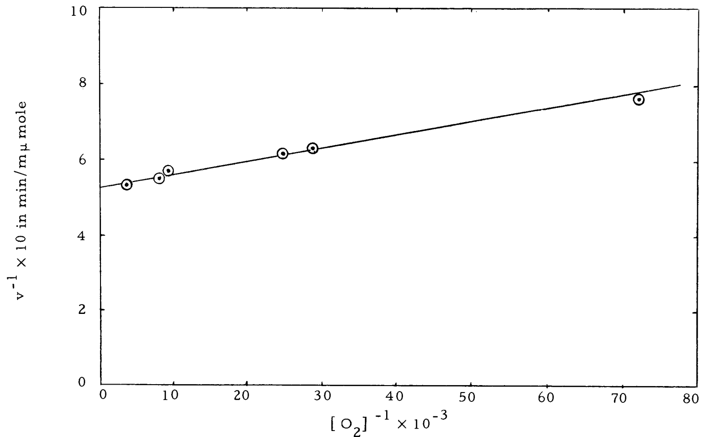
Figure 9. Lineweaver-Burk plot of the influence of oxygen tension on the rate of benzylamine oxidation by plasma amine oxidase (PAO) at pH 7.1. Benzylamine, 330 m \mu mole, and 0.138 mg of PAO were incubated in a total volume of 1.1 ml.
