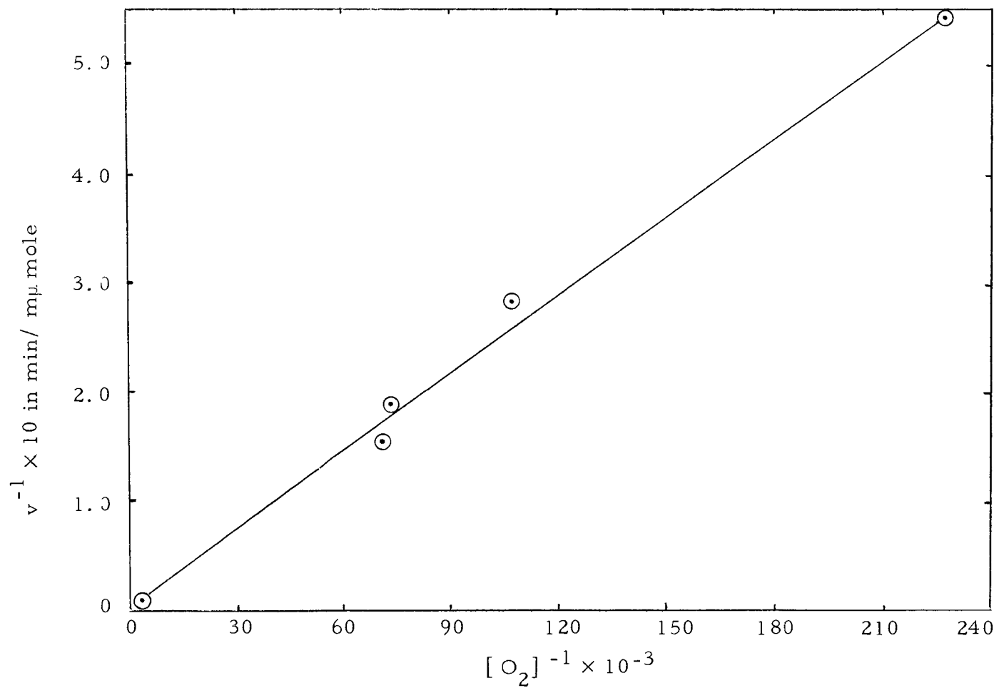
Figure 7. Lineweaver-Burk plot of the influence of oxygen tension on the rate of putrescine oxidation by partially purified diamine oxidase (ppDAO) at pH 8. Putrescine, 210 m\mu moles, and 0.113 mg of ppDAO were incubated in a total volume of 1.1 ml.
