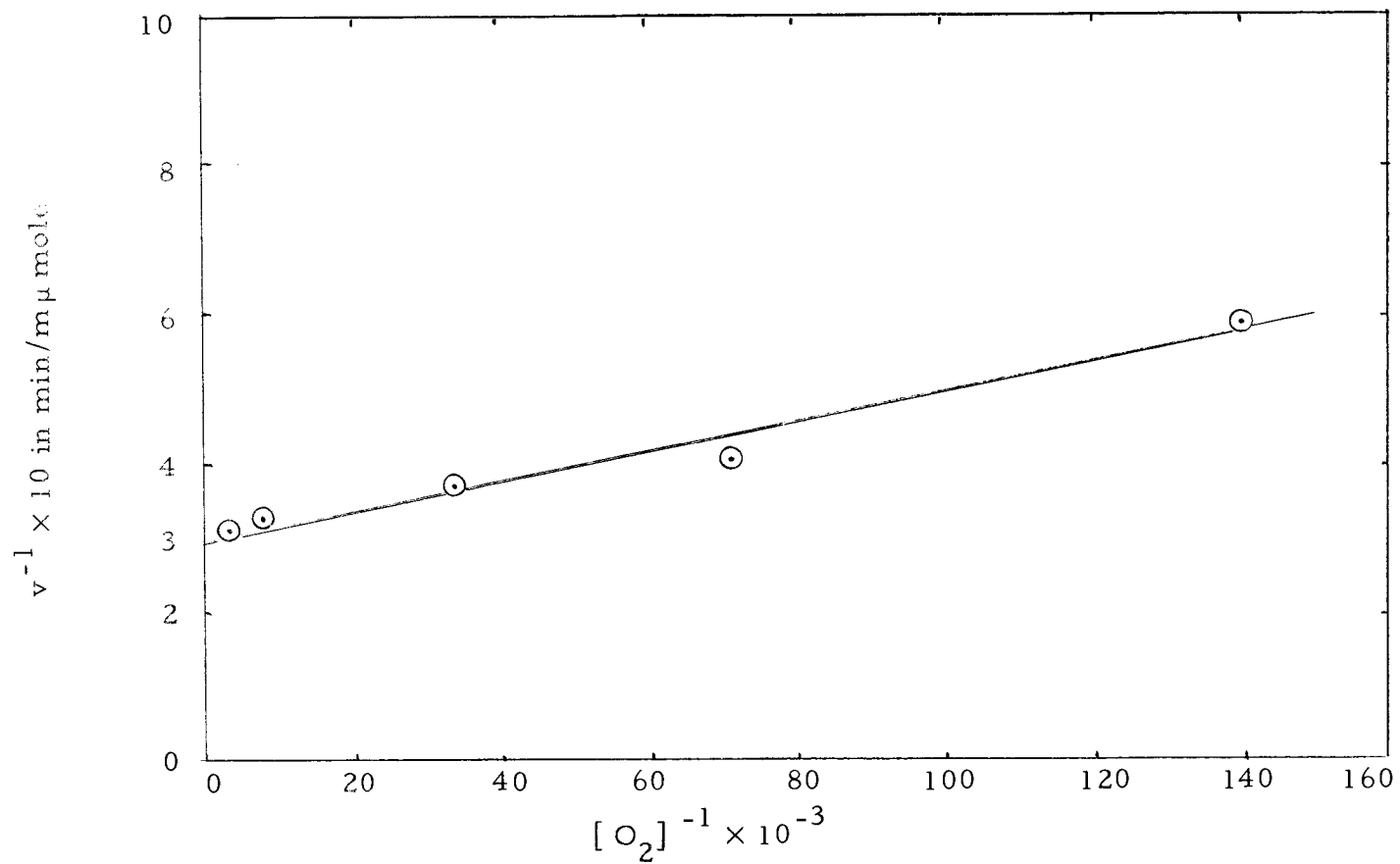
Figure 6. Lineweaver-Burk plot of the influence of oxygen tension on the rate of tryptamine oxidation by partially purified diamine oxidase (ppDAO) at pH 8. Tryptamine, 205 m \mu moles, and 0.113 mg of ppDAO were incubated in a total volume of 1.1 ml.
