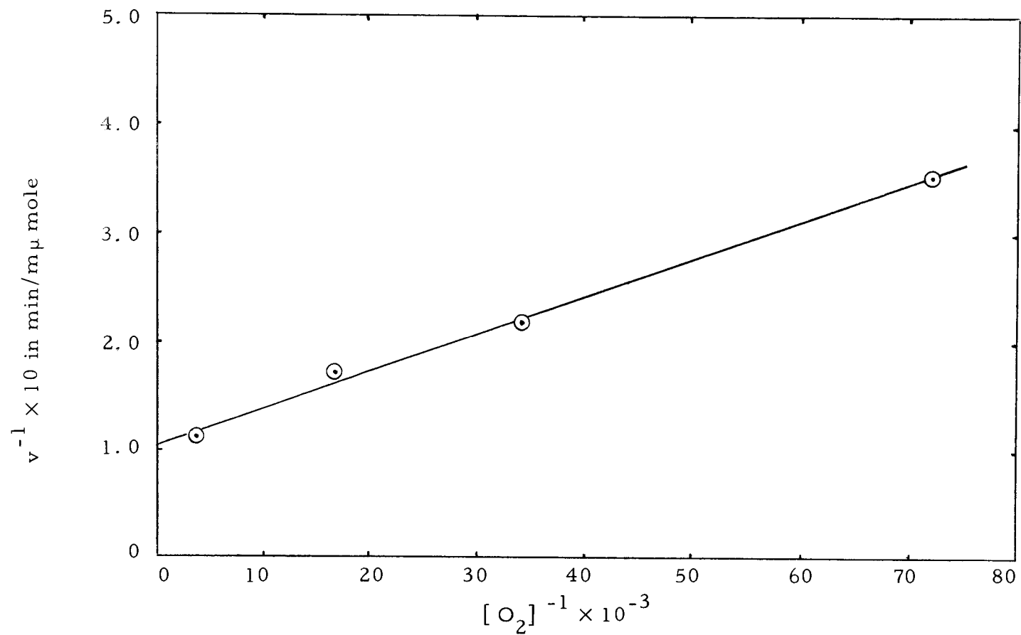
Figure 8. Lineweaver-Burk plot of the influence of oxygen tension on the rate of benzylamine oxidation by plasma amine oxidase (PAO) at pH 7.1. Benzylamine, 3300 m \mu moles, and 0.138 mg of PAO were incubated in a total volume of 1.1 ml.
