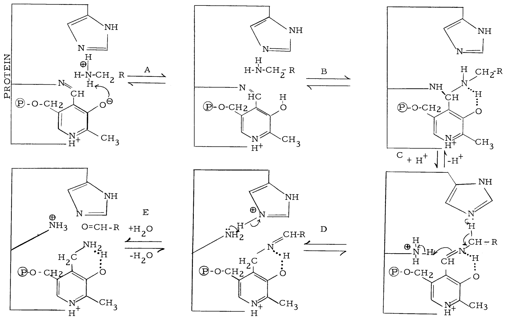
Figure 1. Speculative mechanism for the initial steps of the deamination reaction of rabbit plasma amine oxidase (McEwen, Cullen, and Sober, 1966).
